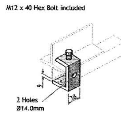
End Cap for Double strut DSSB 6153-2
