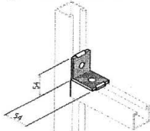
DSSB2806A (WITH KNOCKOUT 2 SIDE) DSSB2806 (WITHOUT KNOCKOUT 2 SIDE)
